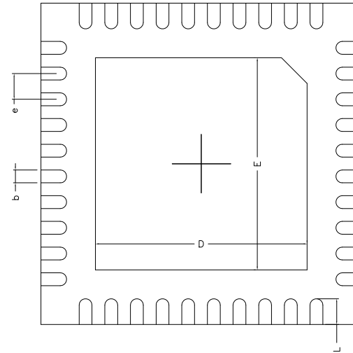
BOTTEM VIEW
