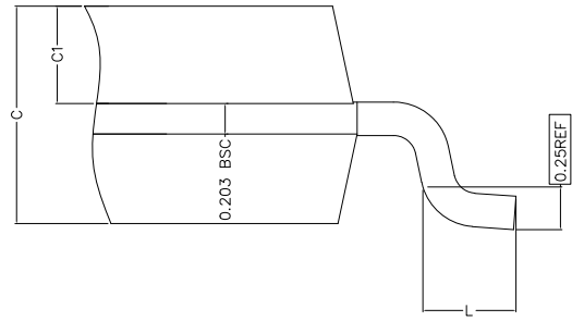
DETAIL E
